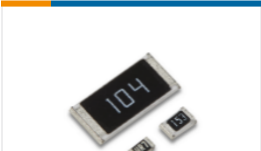
TE Part #1-2176347-3 CRGCQ 2010 100R 1%
